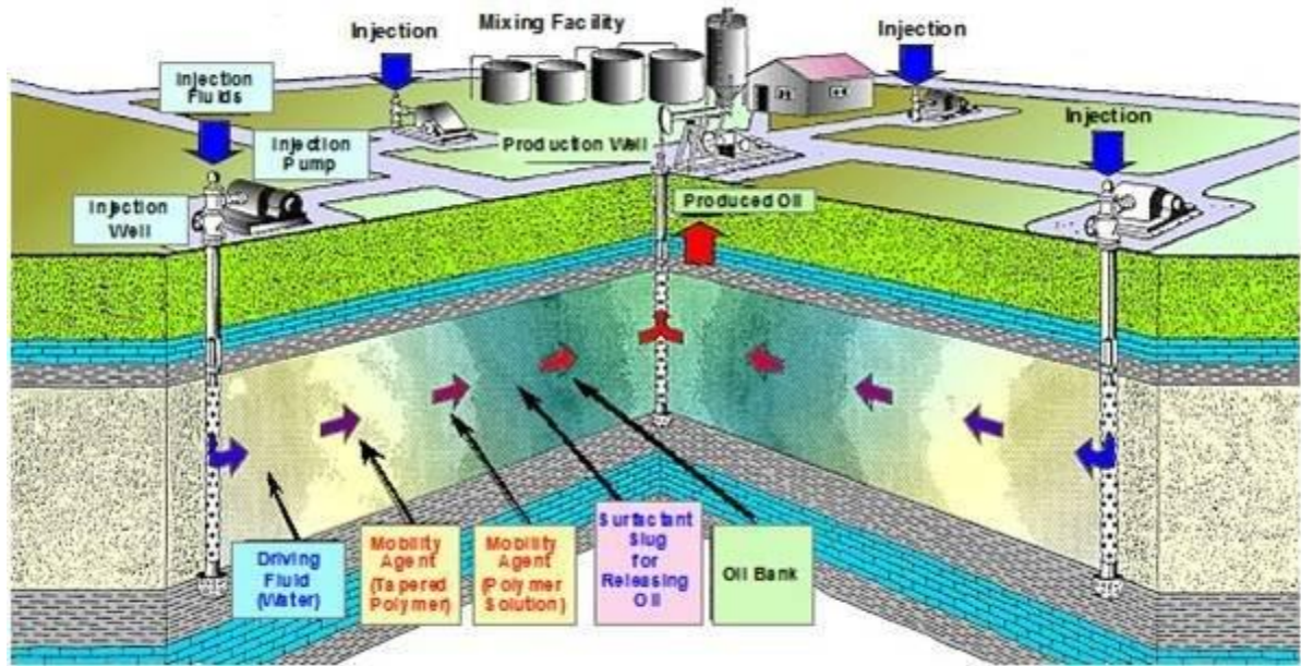
Figure 3 Chemical Flooding
